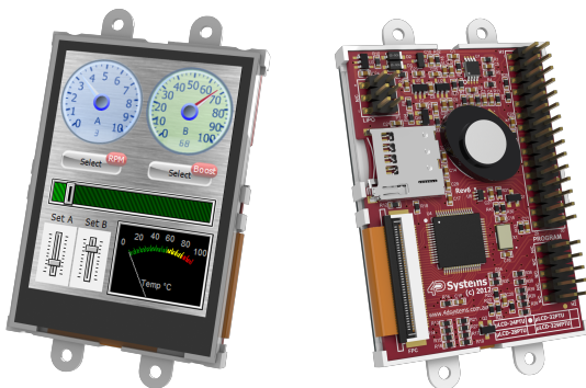
uLCD-24PTU – 2.4" Intelligent PICASO Display
